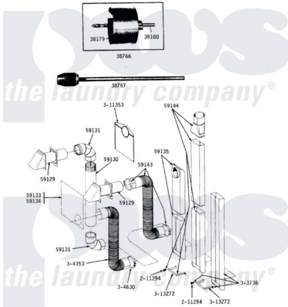
Maytag Residential Maytag DE16CT Dryer Parts Parts Diagram 08 - INSTALLATION ACCESSORIES Click on the part number to view part
