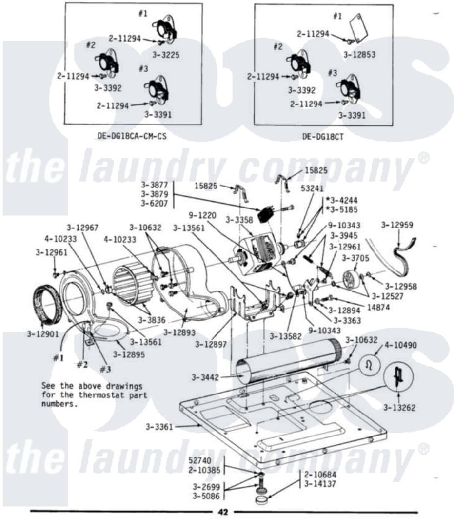
Maytag Residential Maytag DE18CA Dryer Parts Diagram 14 - MOTOR, BLOWER, BASE FRAME & THERMOSTATS
