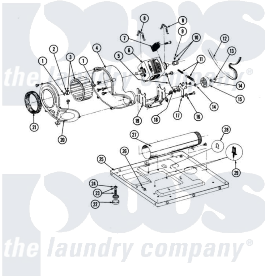
Maytag Residential Maytag DE27CA Dryer Parts Parts Diagram 08 - MOTOR, BLOWER & BASE FRAME Click on the part number to view part
