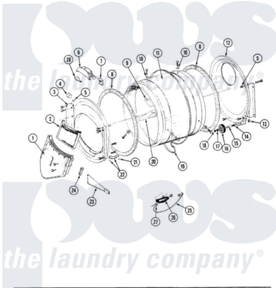
Maytag Residential Maytag DE8300 Dryer Parts Parts Diagram 07 - LINT SCREEN, TUMBLER (FRONT & BACK) Click on the part number to view part
