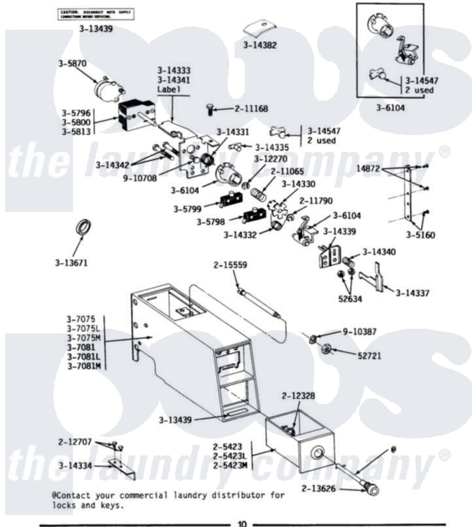
Maytag Residential Maytag DG25CS Dryer Parts Parts Diagram 05 - CONTROL CENTER Click on the part number to view part
