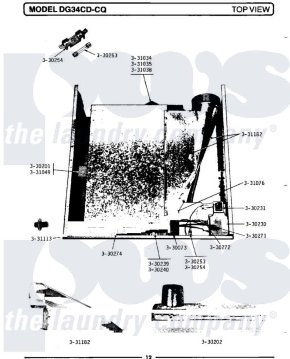
Maytag Residential Maytag DG34CQ Dryer Parts Parts Diagram 06 - TOP VIEW Click on the part number to view part
