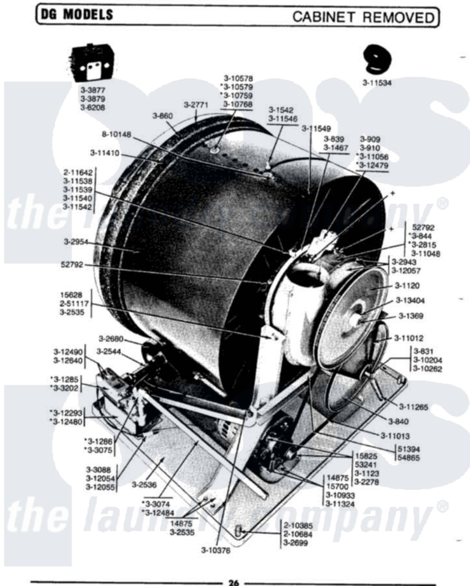
Maytag Residential Maytag DG406 Dryer Parts Parts Diagram 03 - CABINET REMOVED Click on the part number to view part
