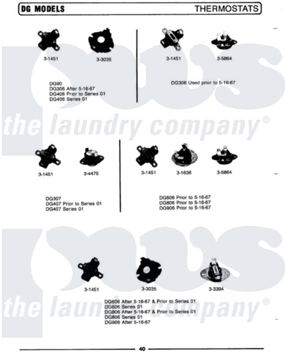
Maytag Residential Maytag DG606 Dryer Parts Parts Diagram 11 - THERMOSTATS Click on the part number to view part
