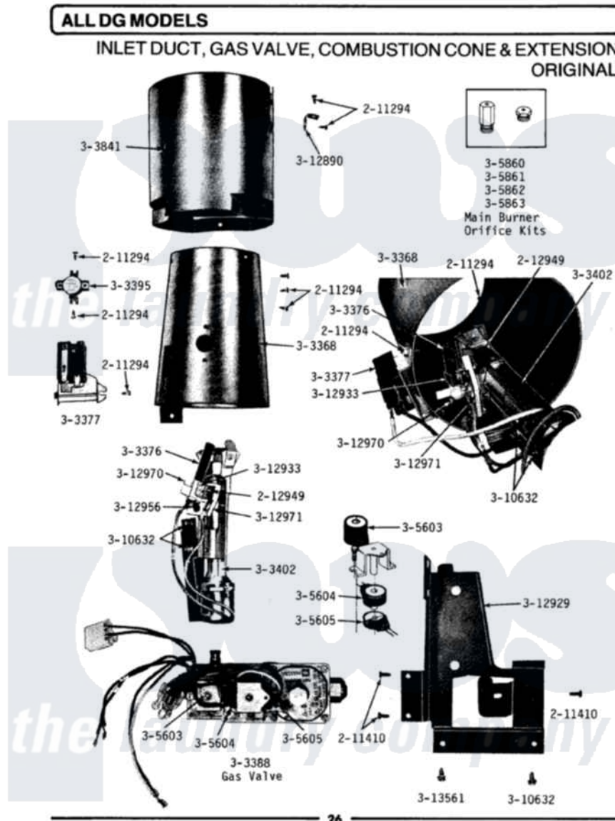
Maytag Residential Maytag DG808 Dryer Parts Parts Diagram 05 - INLET DUCT, GAS VALVE, CONE & EXTENSION Click on the part number to view part
