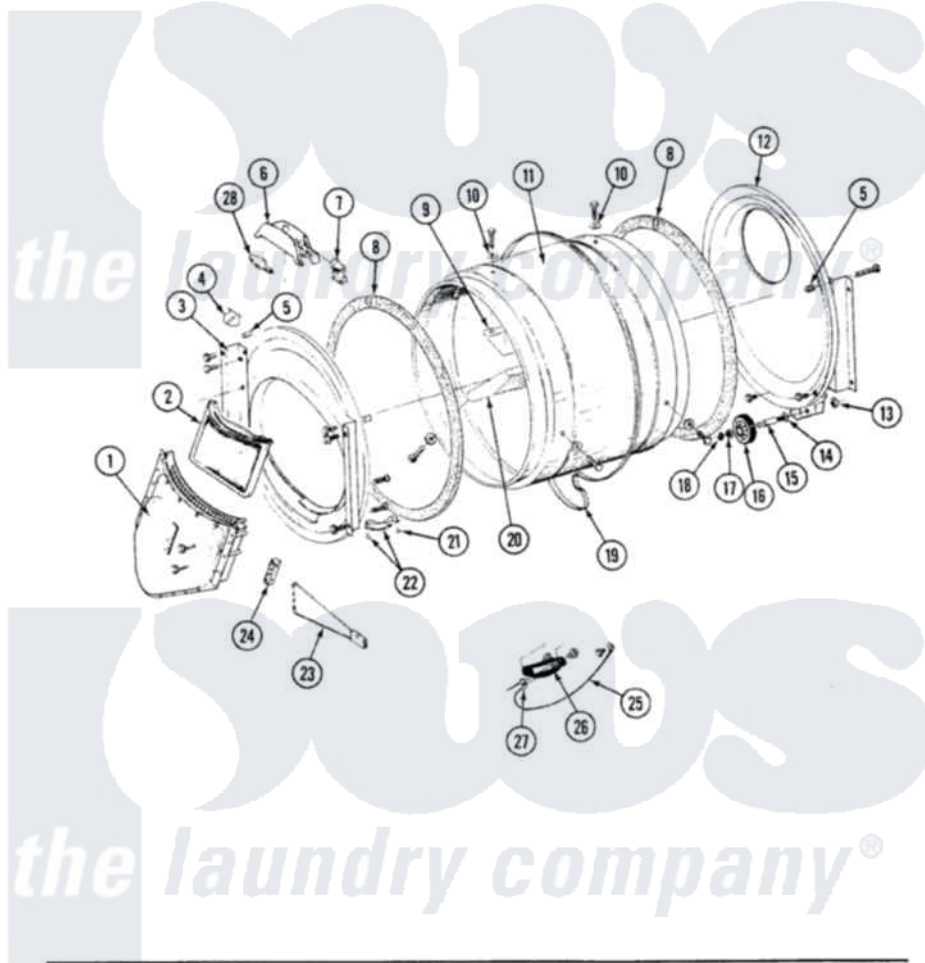
Maytag Residential Maytag DG9800 Dryer Parts Parts Diagram 06 - LINT SCREEN, TUMBLER (FRONT & BACK) Click on the part number to view part
