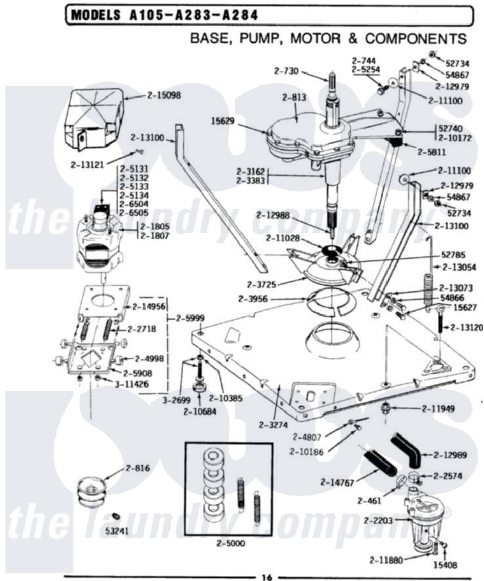
Maytag Residential Maytag GA283 Washer Parts Parts Diagram 01 - BASE, PUMP, MOTOR & COMPONENTS Click on the part number to view part
