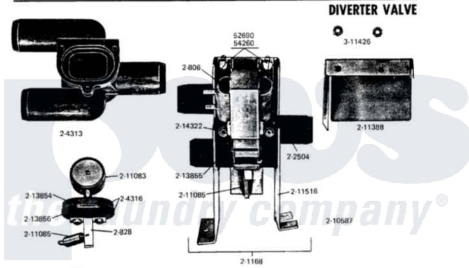
Maytag Residential Maytag GA608 Washer Parts Parts Diagram 02 - BLEACH INJECTION SYSTEM Click on the part number to view part
