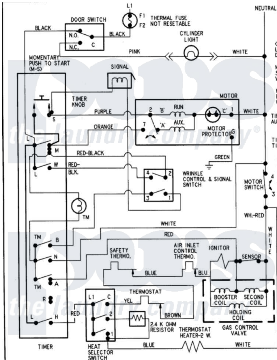
Maytag Residential Maytag HYG3460AWW Dryer Parts Parts Diagram 09 - WIRING INFORMATION Click on the part number to view part
