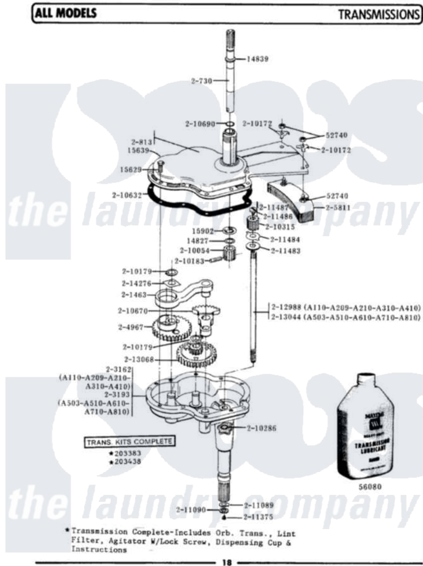
Maytag Residential Maytag LA209S Washer Parts Parts Diagram 07 - TRANSMISSIONS Click on the part number to view part
