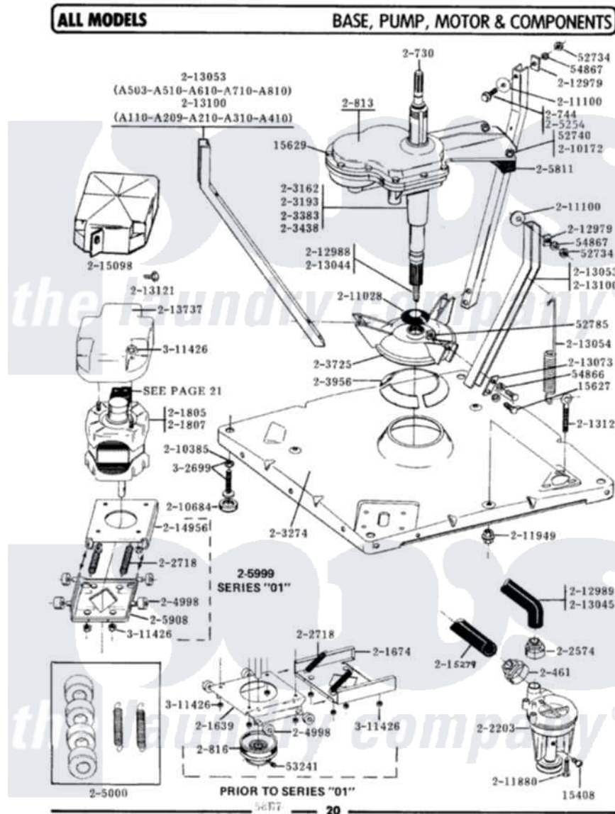
Maytag Residential Maytag LA210S Washer Parts Parts Diagram 01 - BASE\PUMP\MOTOR Click on the part number to view part
