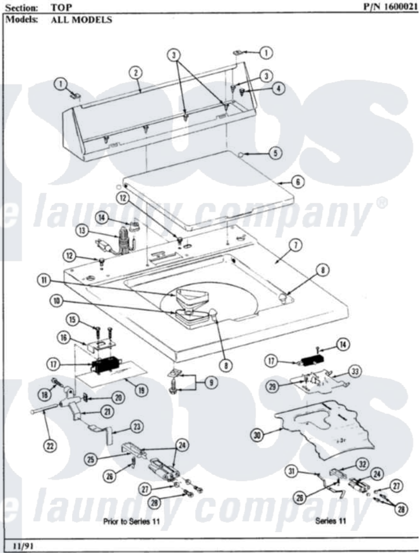
Maytag Residential Maytag LA482 Washer Parts Parts Diagram 06 - TOP Click on the part number to view part
