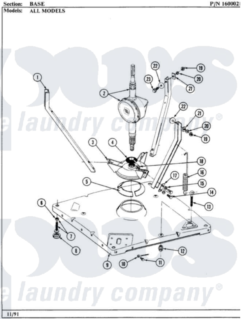
Maytag Residential Maytag LA484 Washer Parts Parts Diagram 01 - BASE Click on the part number to view part
