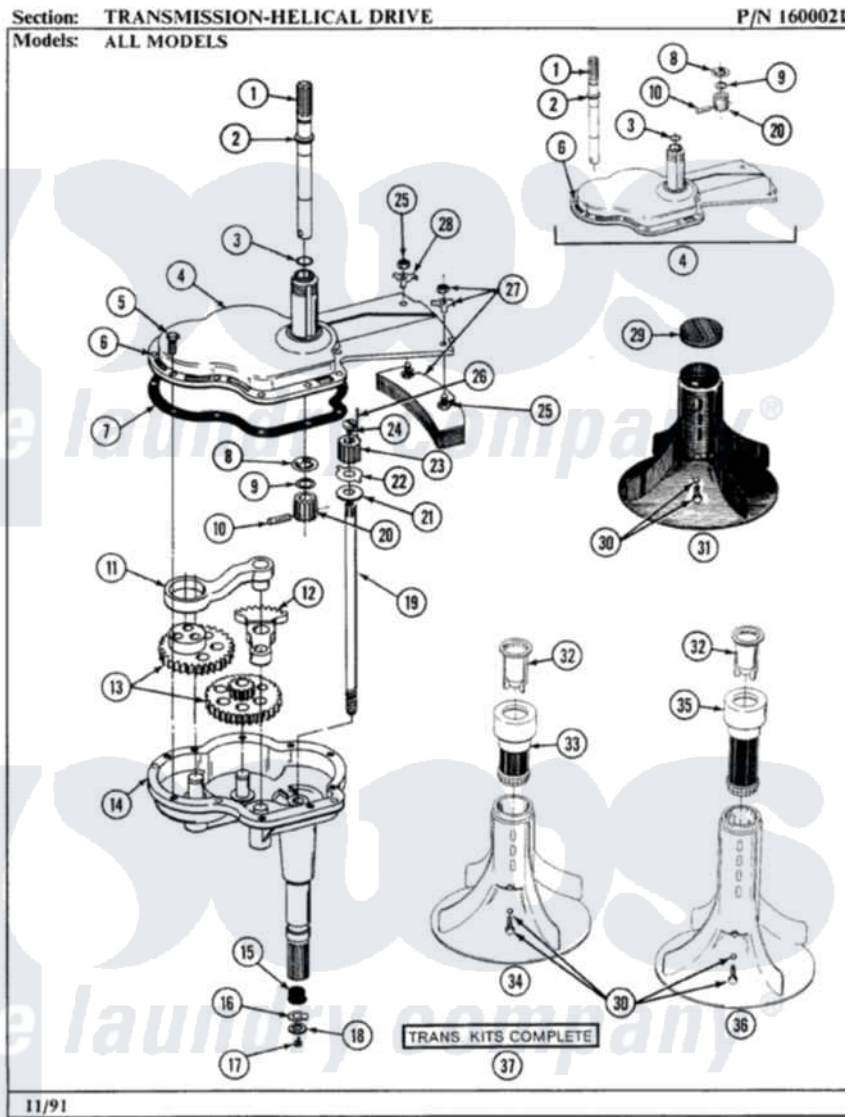
Maytag Residential Maytag LA884 Washer Parts Parts Diagram 07 - TRANSMISSION-HELICAL DRIVE Click on the part number to view part
