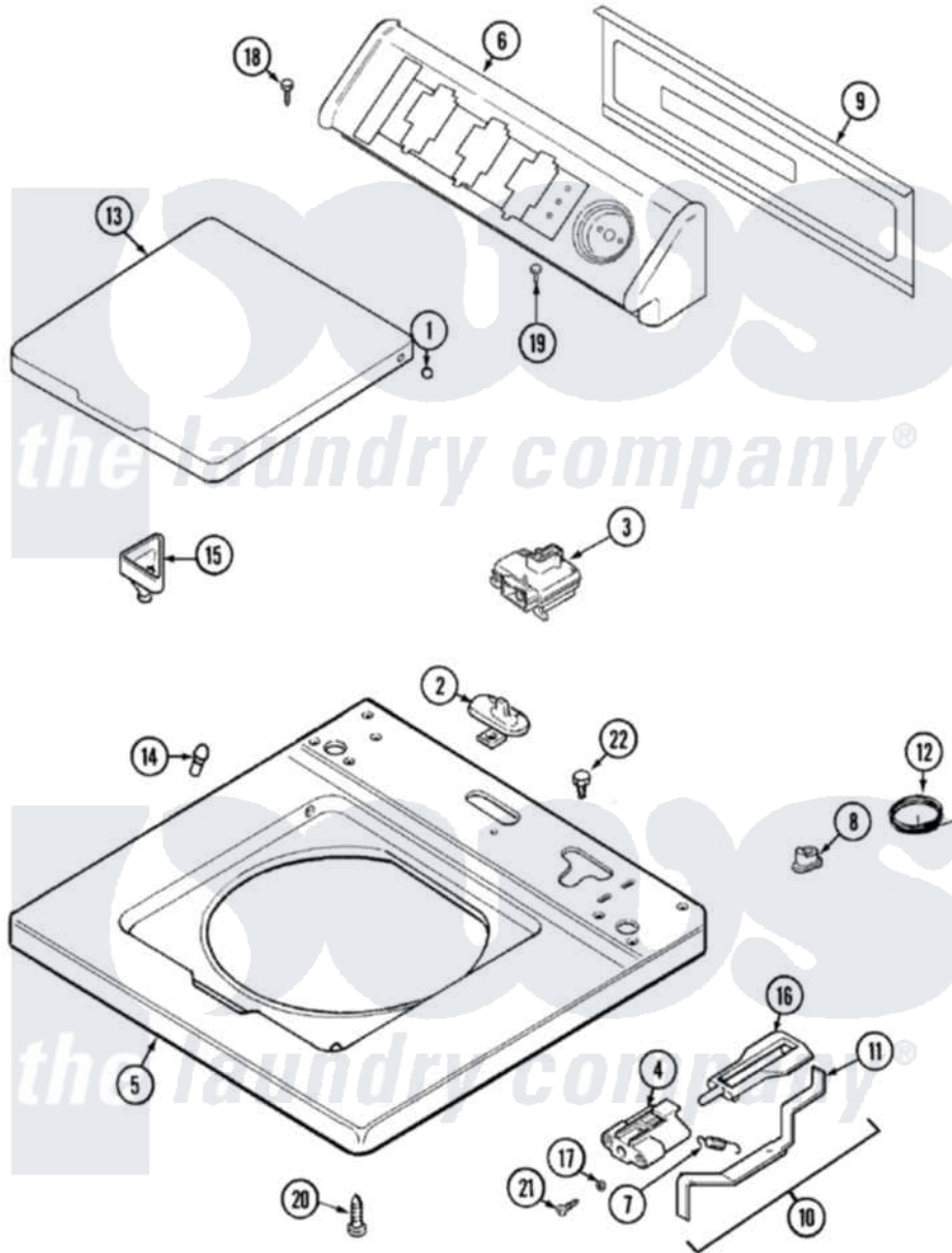
Maytag Residential Maytag LAT2301AAE Washer Parts Parts Diagram 06 - TOP Click on the part number to view part
