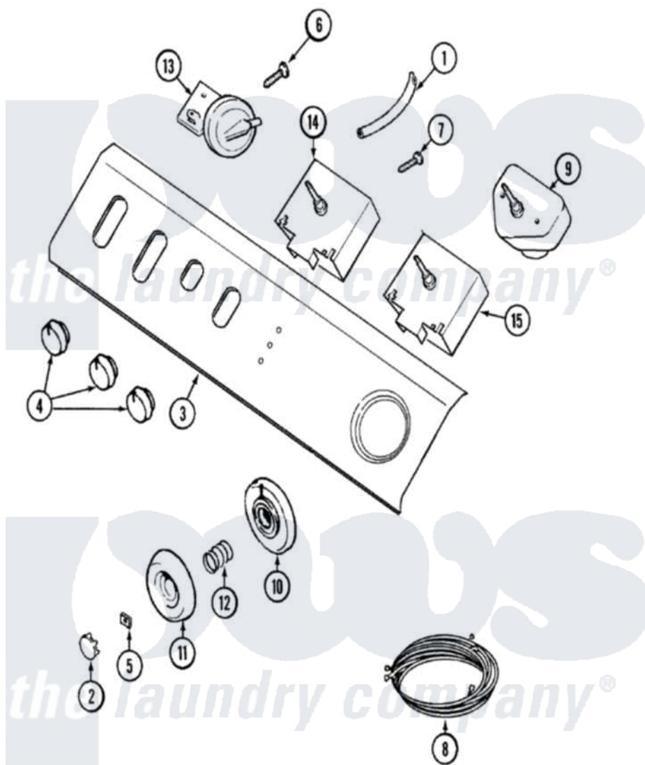
Maytag Residential Maytag LAT4916ABE Washer Parts Parts Diagram 04 - CONTROL PANEL
