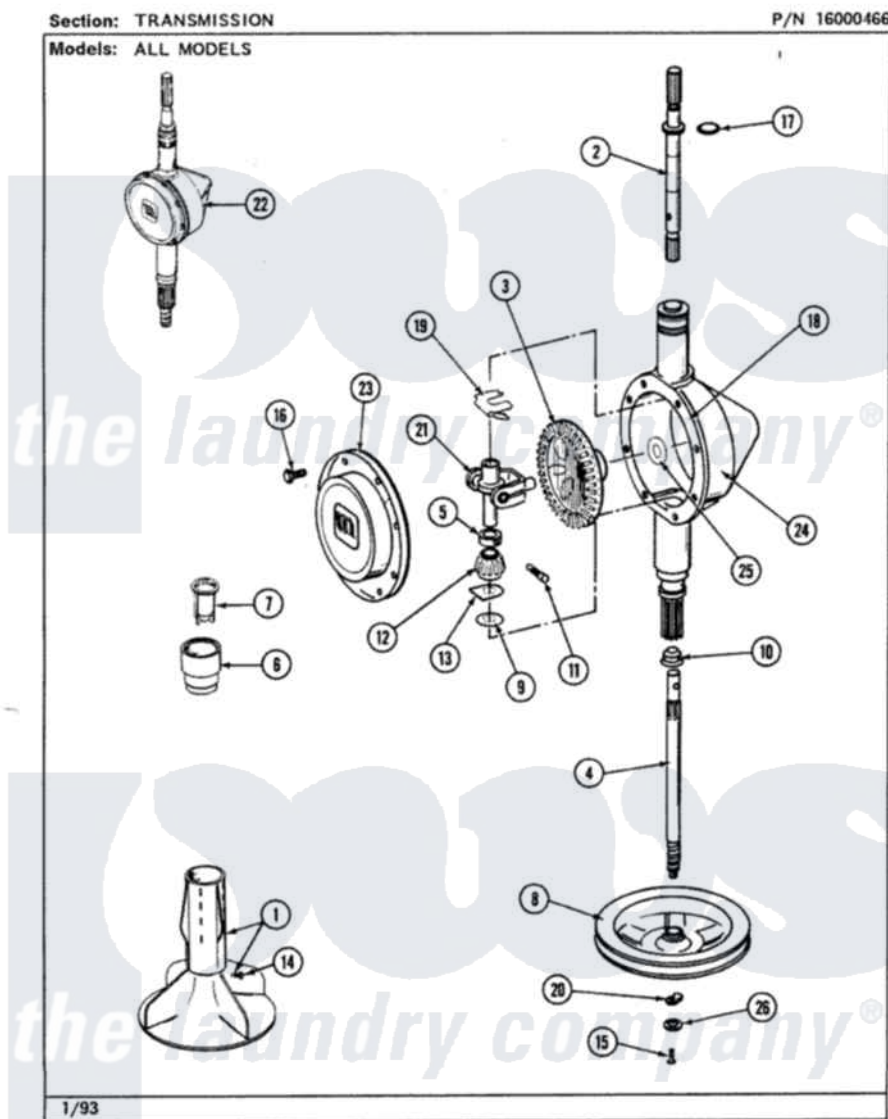
Maytag Residential Maytag LAT7793AAL Washer Parts Parts Diagram 06 - TRANSMISSION Click on the part number to view part
