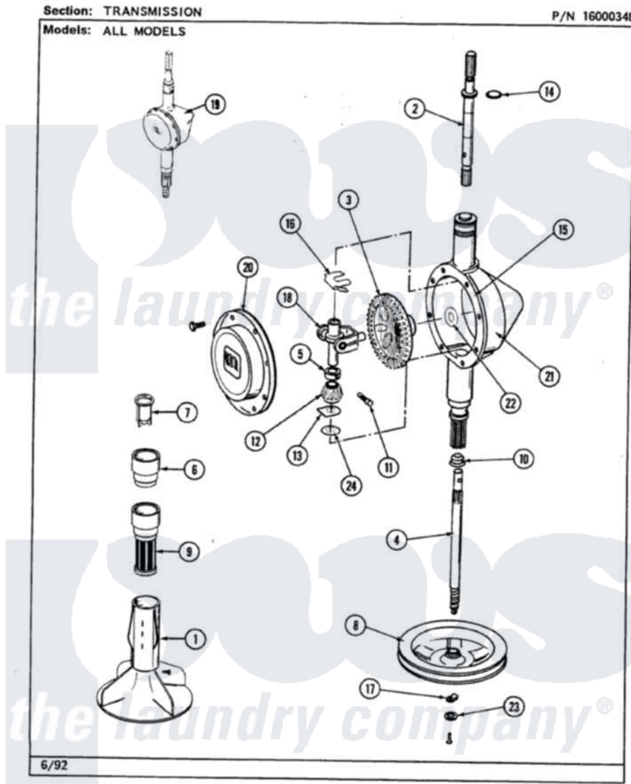
Maytag Residential Maytag LAT7800AAW Washer Parts Parts Diagram 06 - TRANSMISSION Click on the part number to view part
