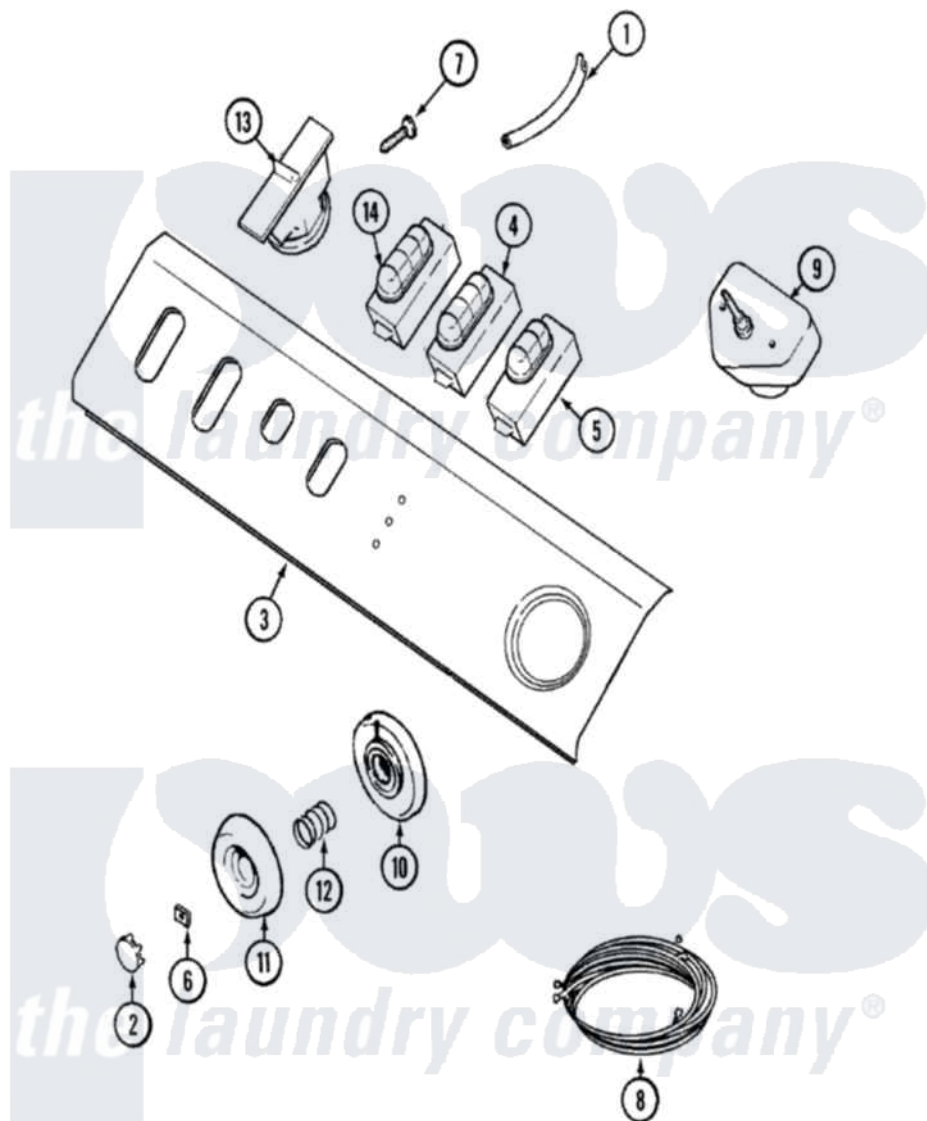
Maytag Residential Maytag LAT8706AAE Washer Parts Parts Diagram 04 - CONTROL PANEL
