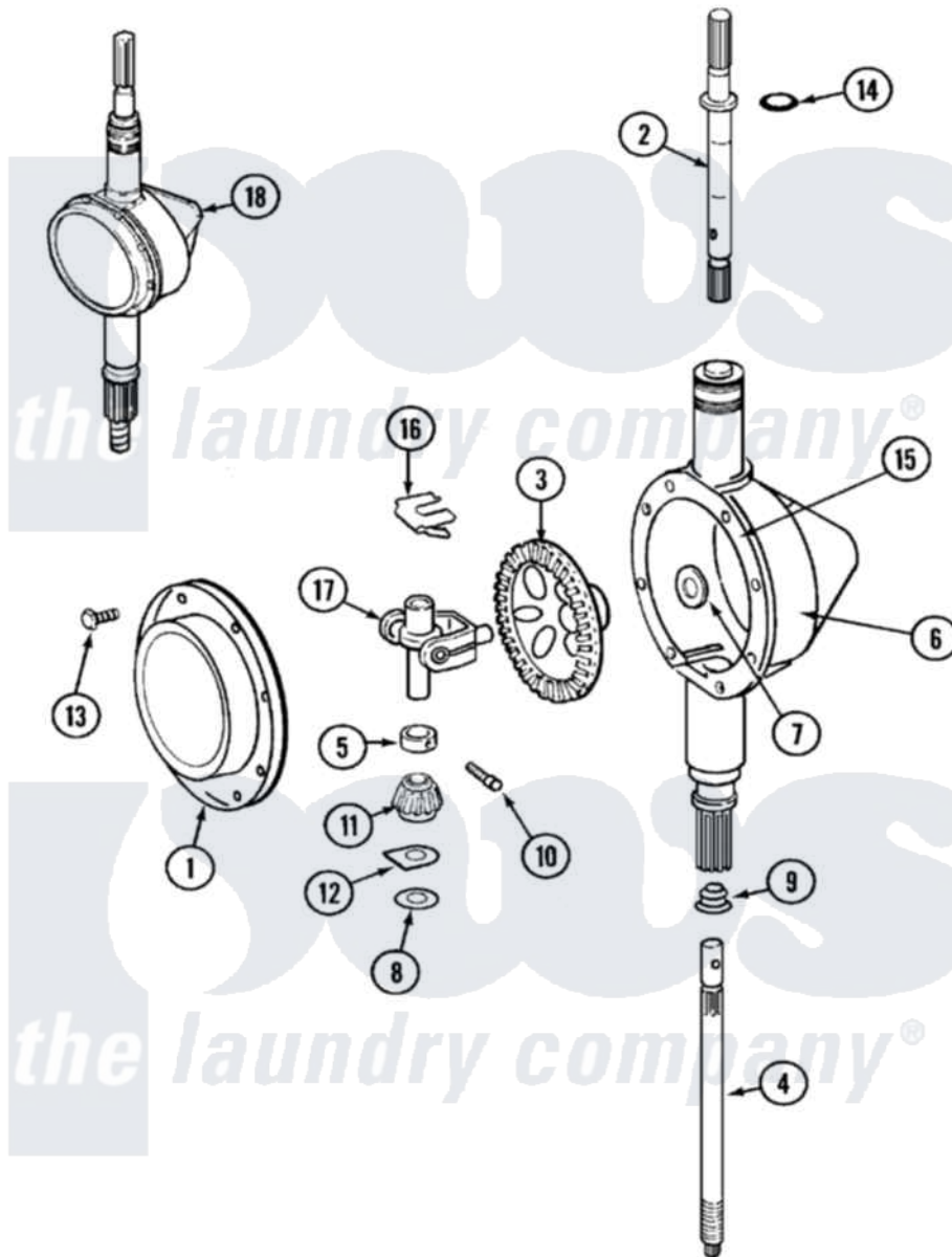
Maytag Residential Maytag LAT9304DAM Washer Parts Parts Diagram 06 - TRANSMISSION (LAW9304AAM & LAT9304DAM)
