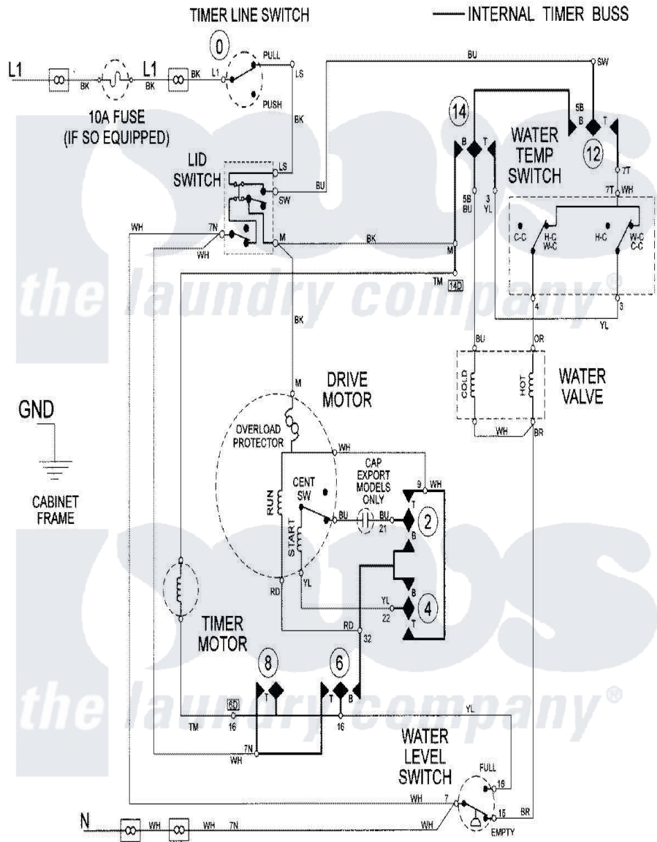
Maytag Residential Maytag LAT9306AKQ Washer Parts Parts Diagram 08 - WIRING INFO (LAT9306DAM/AKQ/DAQ)(SER 10) Click on the part number to view part
