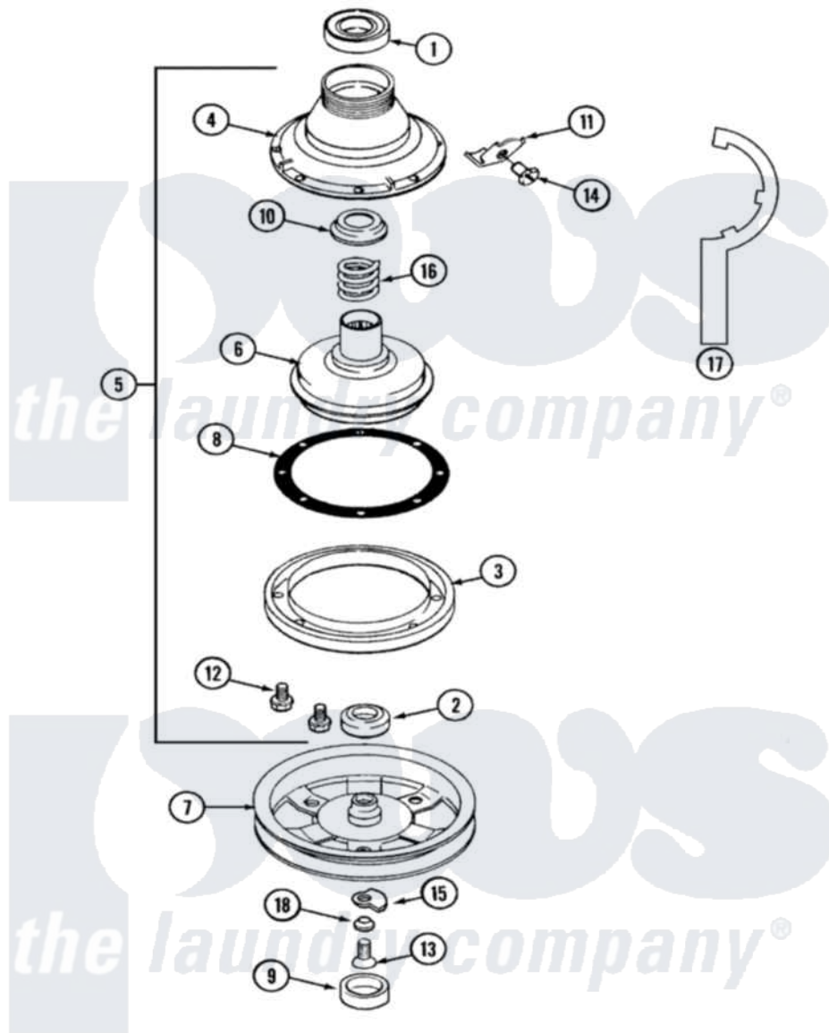
Maytag Residential Maytag LAT9357AAE Washer Parts Parts Diagram 03 - CLUTCH, BRAKE & BELTS
