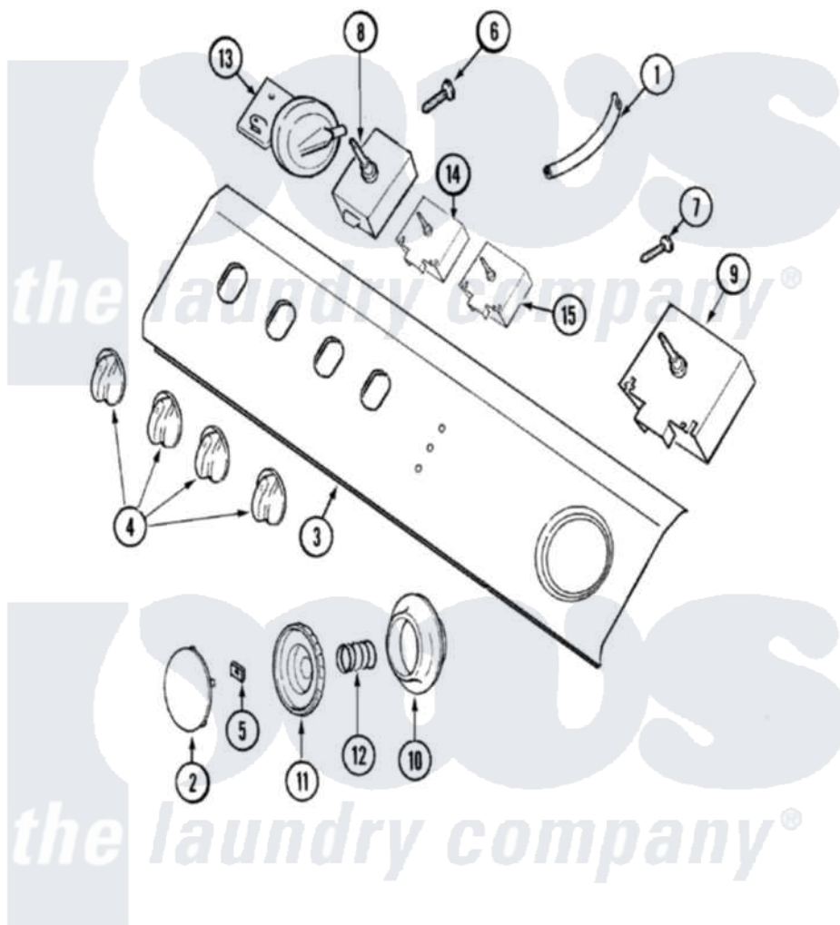
Maytag Residential Maytag LAT9457BAE Washer Parts Parts Diagram 04 - CONTROL PANEL Click on the part number to view part
