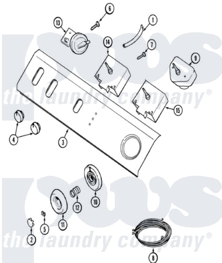
Maytag Residential Maytag LAT9520AAE Washer Parts Parts Diagram 04 - CONTROL PANEL
