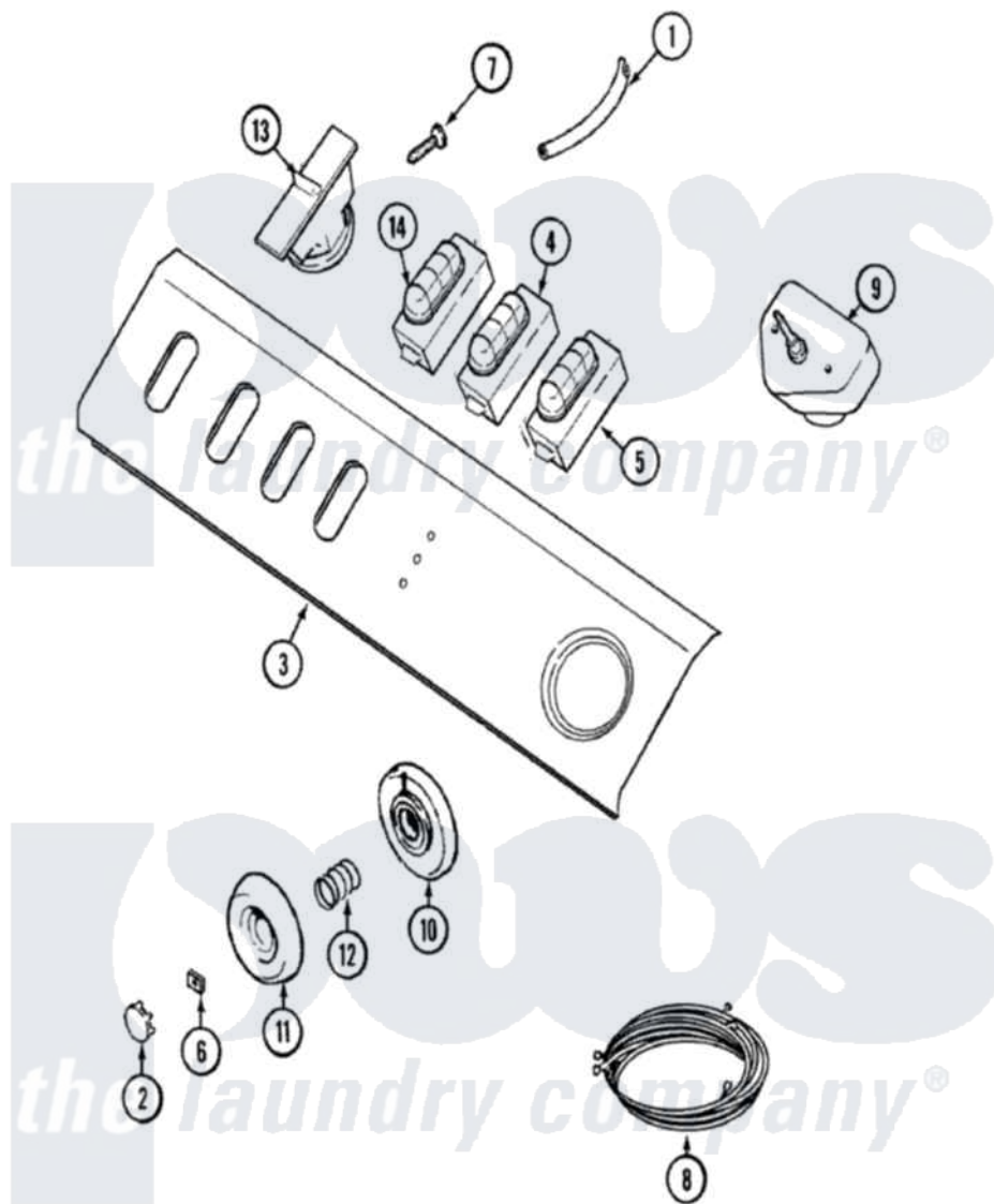
Maytag Residential Maytag LAT9606BGE Washer Parts Parts Diagram 04 - CONTROL PANEL
