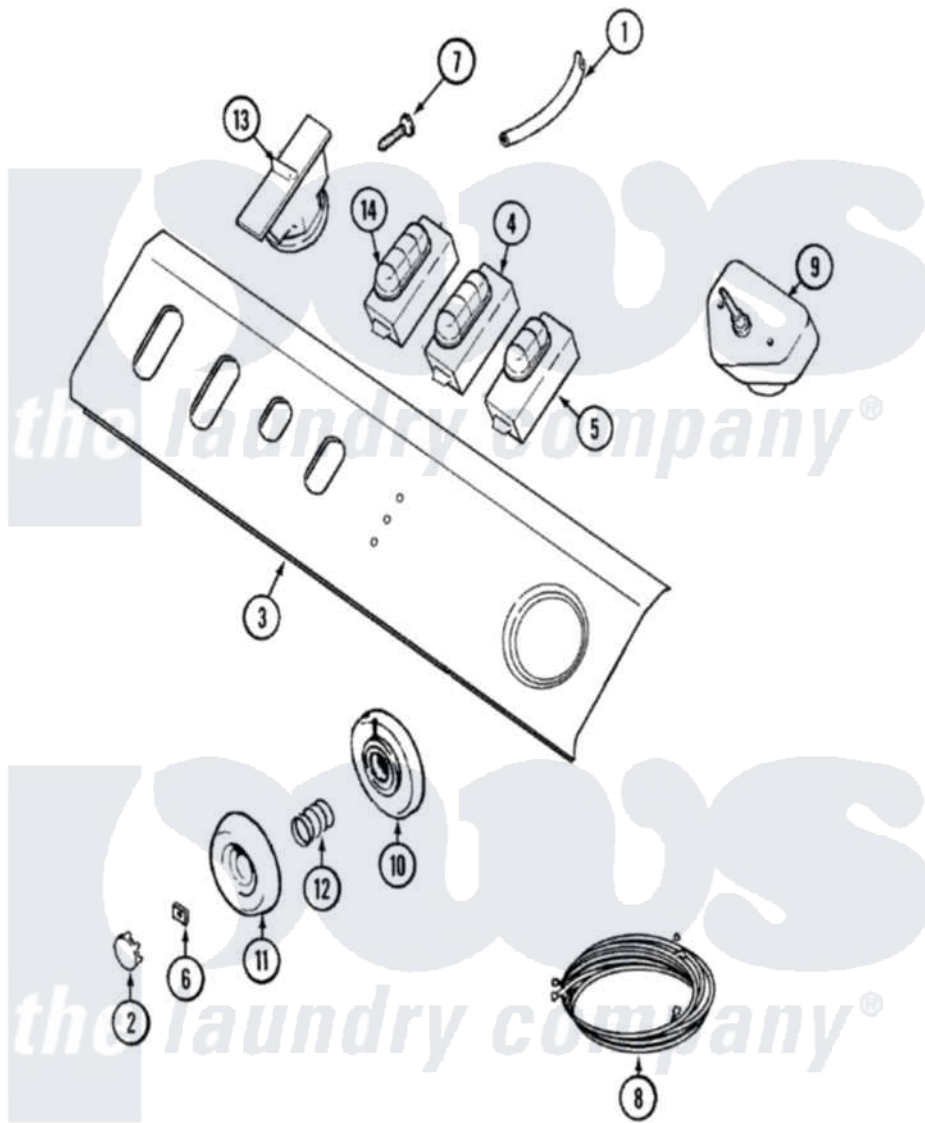
Maytag Residential Maytag LAT9806AAM Washer Parts Parts Diagram 04 - CONTROL PANEL (9806)
