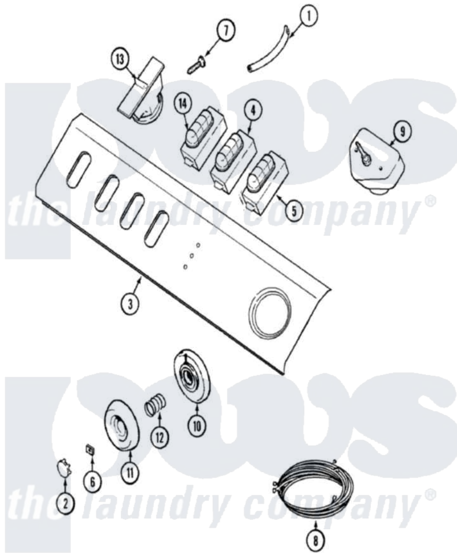
Maytag Residential Maytag LAT9806BGE Washer Parts Parts Diagram 04 - CONTROL PANEL Click on the part number to view part
