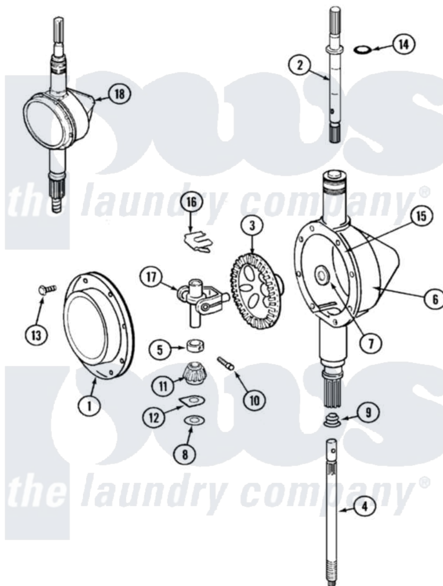
Maytag Residential Maytag LAW9304AAM Washer Parts Parts Diagram 06 - TRANSMISSION (LAW9304AAM & LAT9304DAM)
