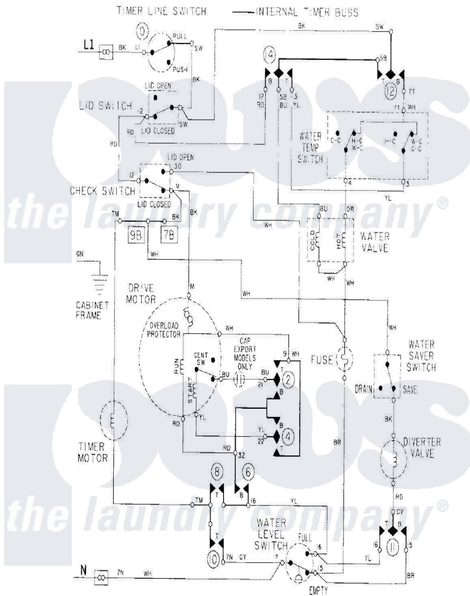
Maytag Residential Maytag LAW9304AAM Washer Parts Parts Diagram 09 - WIRING INFORMATION LAW9304AAx
