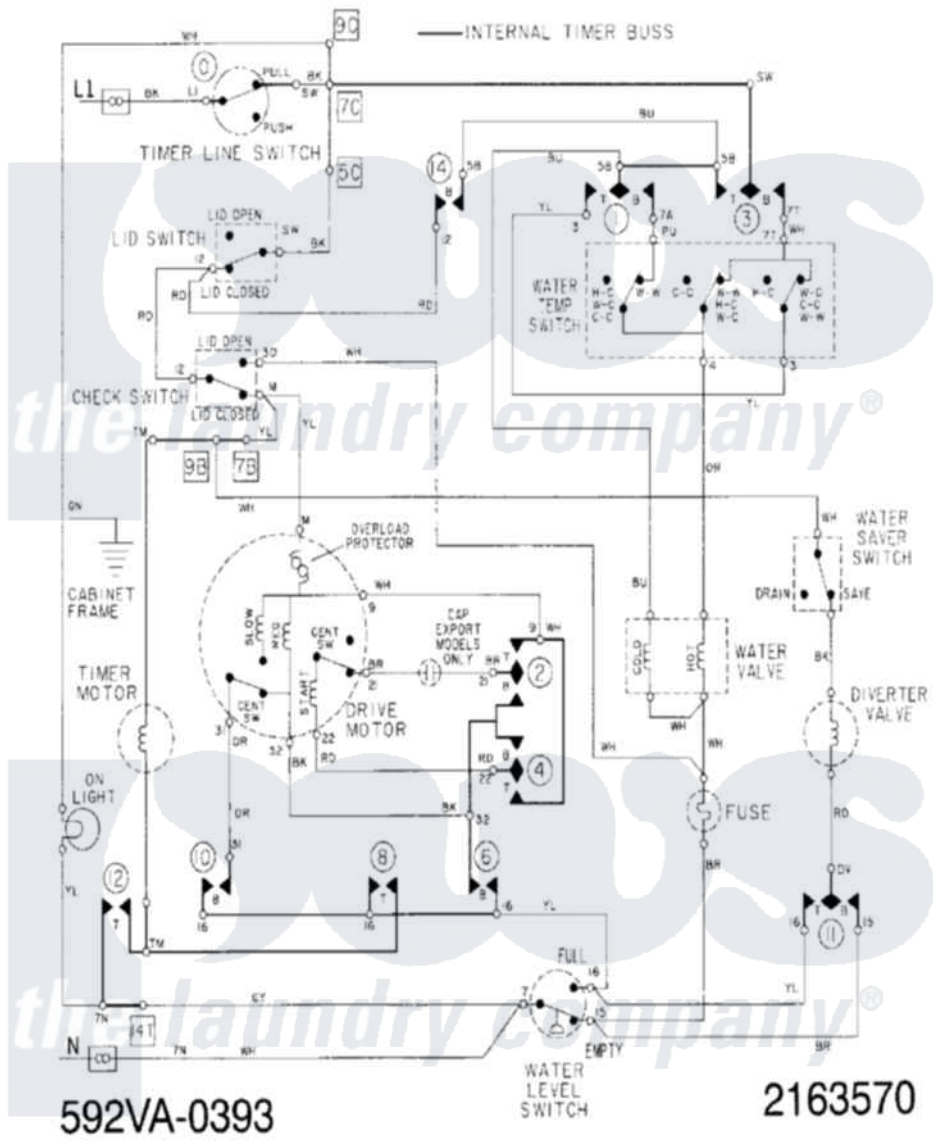
Maytag Residential Maytag LAW9704AAL Washer Parts Parts Diagram 09 - WIRING INFORMATION (LAW9704AAx)
