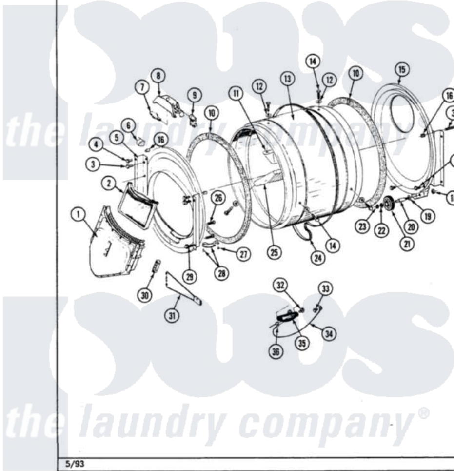
Maytag Residential Maytag LDE4910ACL Dryer Parts Parts Diagram 08 - TUMBLER Click on the part number to view part
