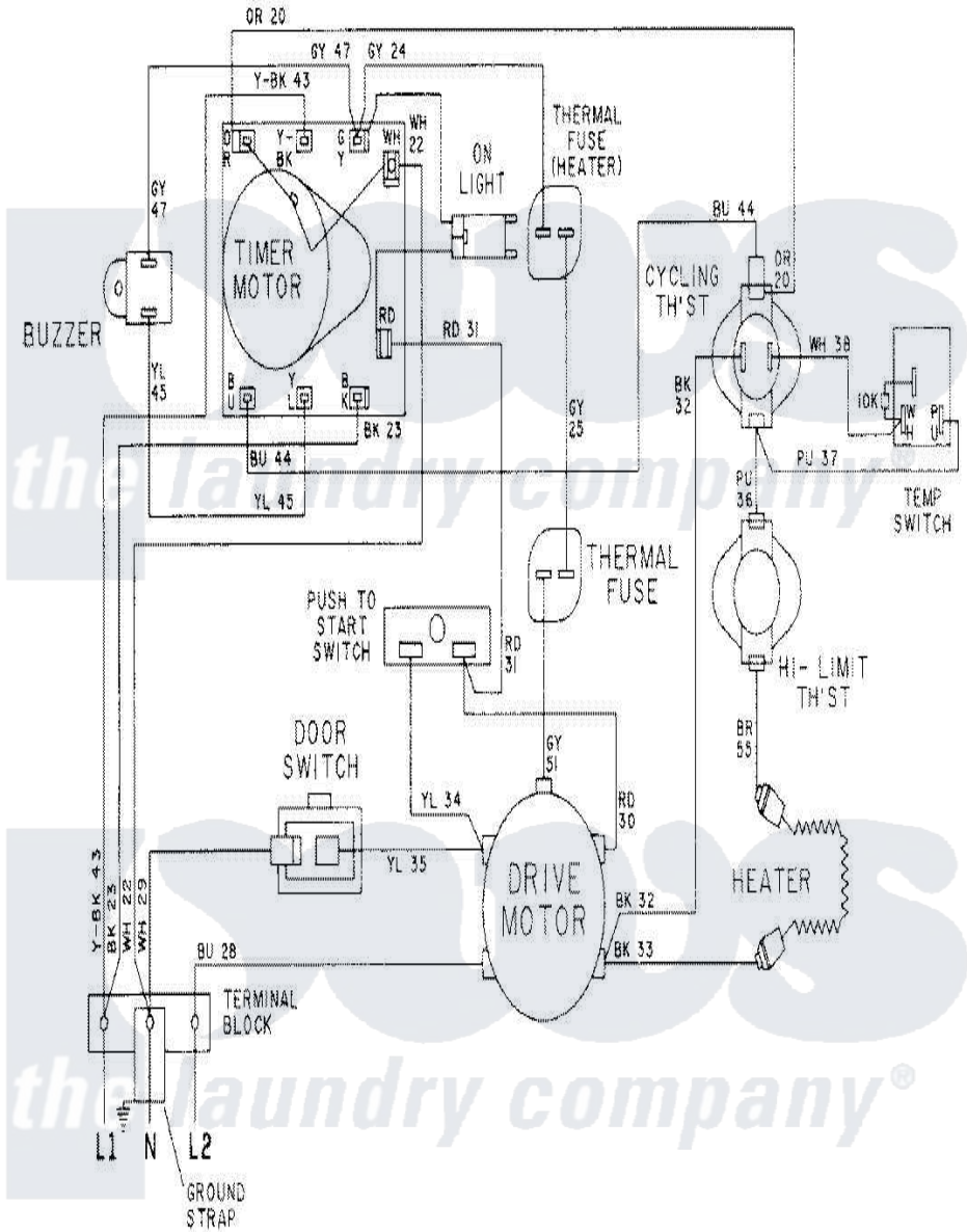
Maytag Residential Maytag LDE7314ACL Dryer Parts Parts Diagram 08 - WIRING INFORMATION-LDE7314ACx Click on the part number to view part
