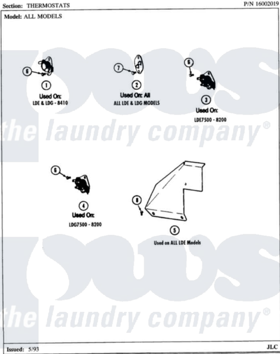
Maytag Residential Maytag LDE7500ACL Dryer Parts Parts Diagram 14 - THERMOSTATS (LDE7500ACM,ADM) & (LDG)
