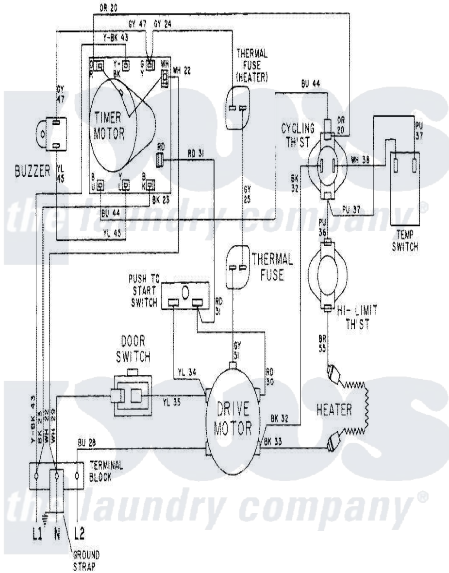
Maytag Residential Maytag LDE8304ACE Dryer Parts Parts Diagram 08 - WIRING INFORMATION-LDE8304ACx Click on the part number to view part
