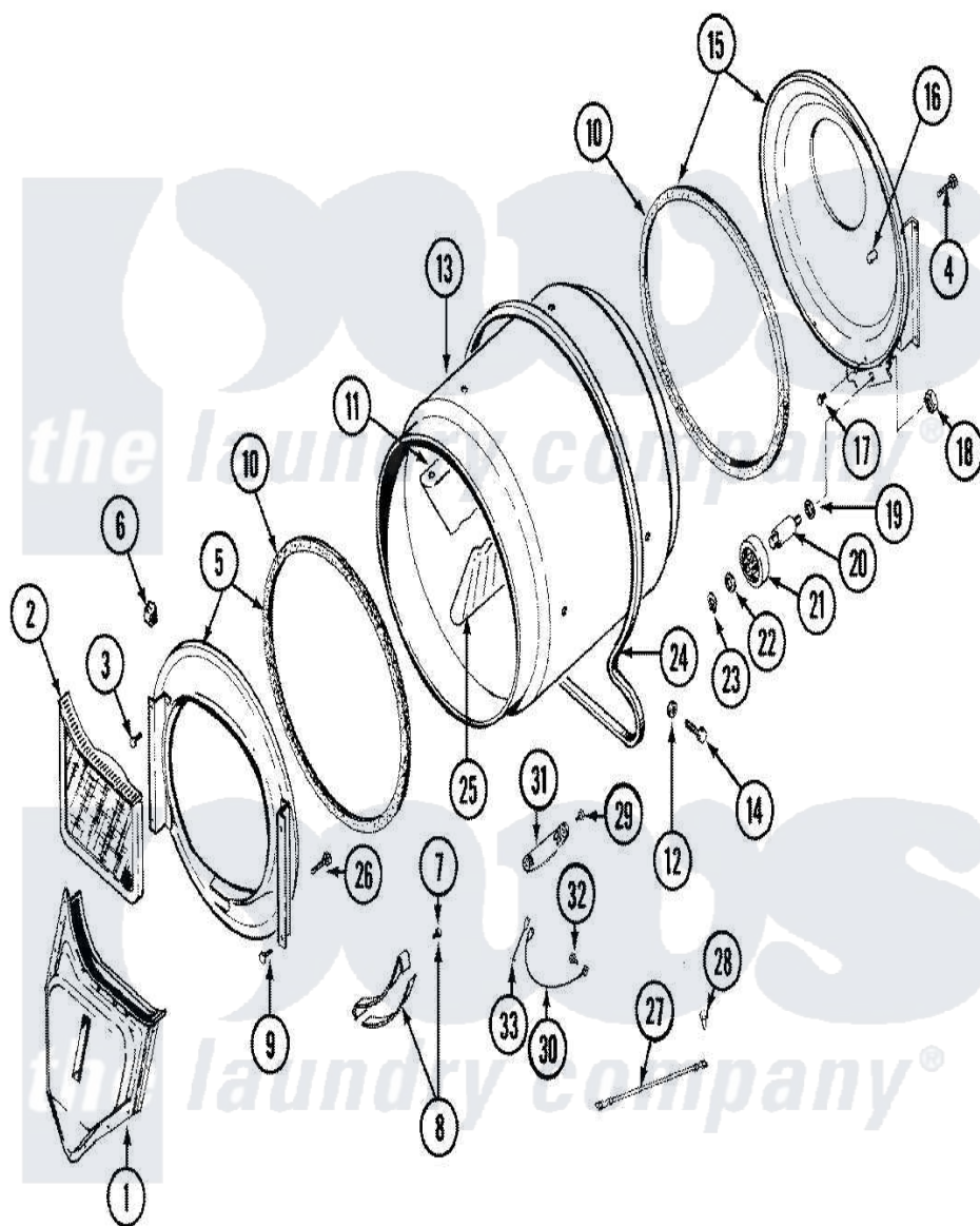
Maytag Residential Maytag LDE8604ACE Dryer Parts Parts Diagram 07 - TUMBLER Click on the part number to view part
