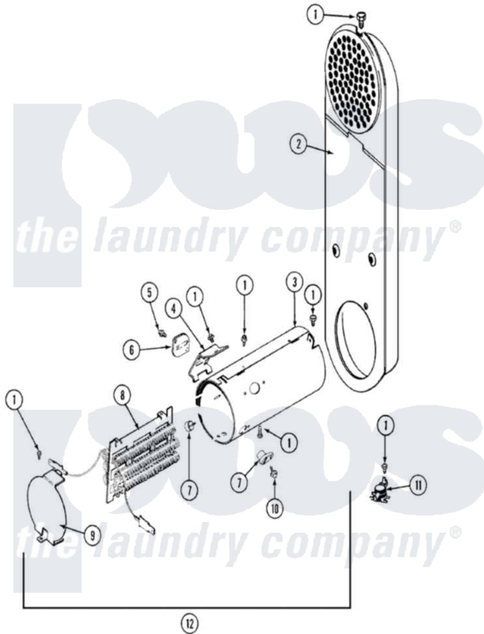
Maytag Residential Maytag LDE8604ACM Dryer Parts Parts Diagram 06 - HEATER Click on the part number to view part
