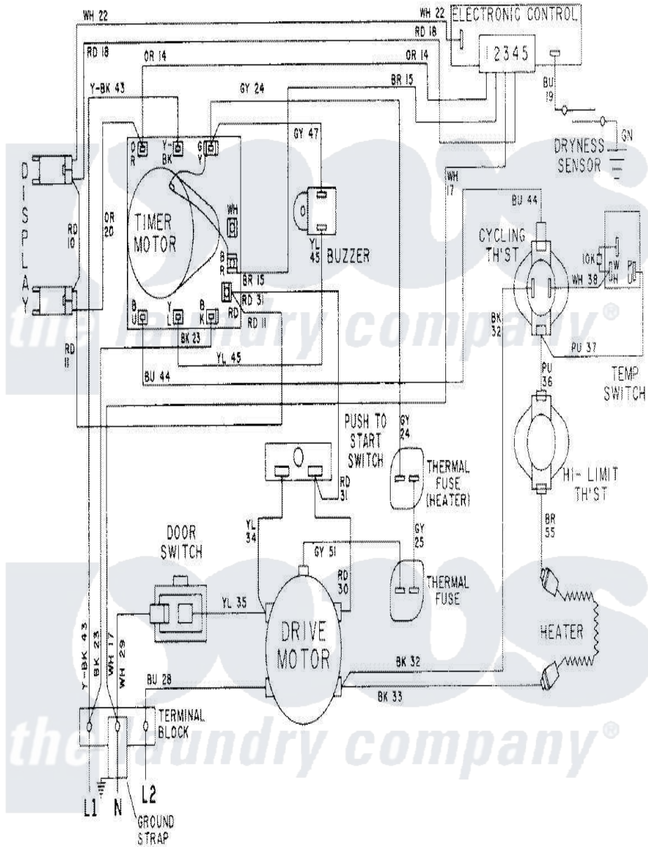
Maytag Residential Maytag LDE8704ACM Dryer Parts Parts Diagram 08 - WIRING INFORMATION-LDE8704ACx Click on the part number to view part
