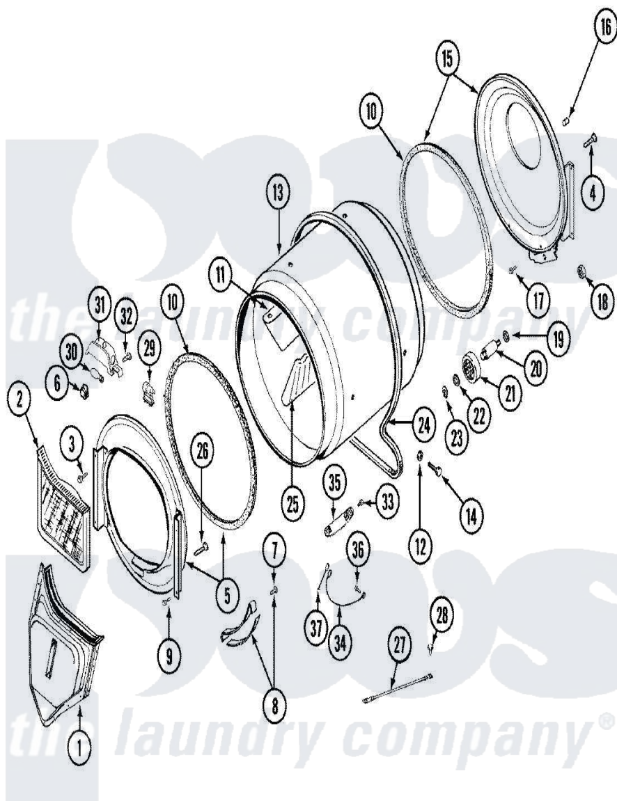
Maytag Residential Maytag LDE8804ACE Dryer Parts Parts Diagram 07 - TUMBLER Click on the part number to view part
