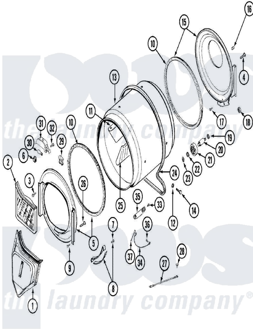
Maytag Residential Maytag LDE9304ACL Dryer Parts Parts Diagram 06 - TUMBLER Click on the part number to view part
