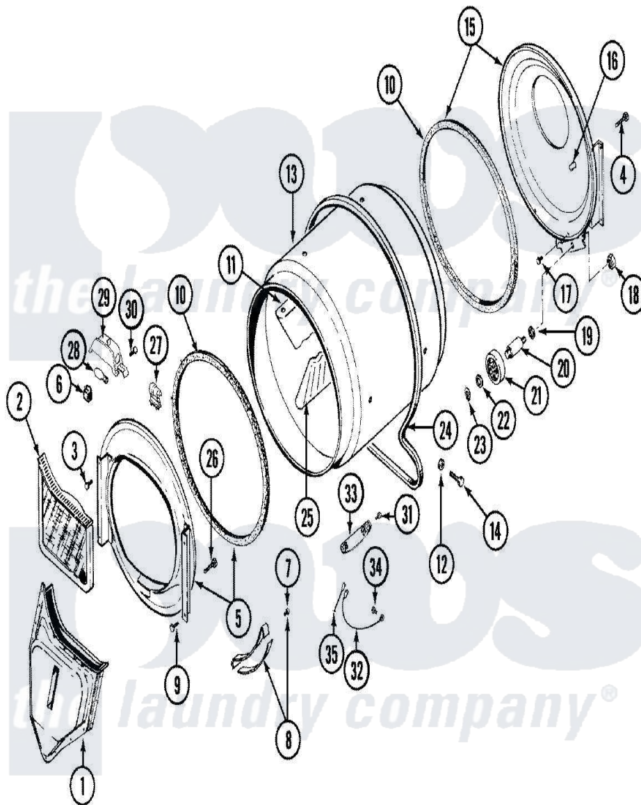
Maytag Residential Maytag LDE9304ADE Dryer Parts Parts Diagram 08 - TUMBLER Click on the part number to view part
