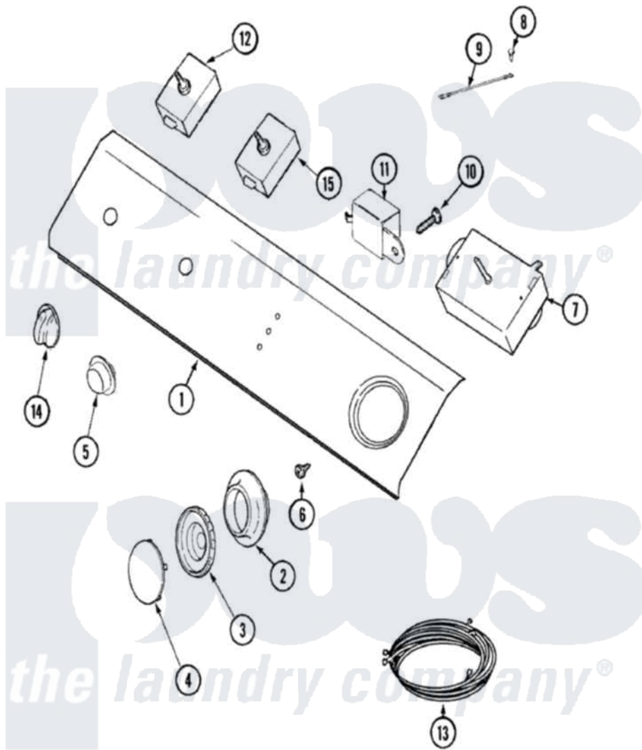
Maytag Residential Maytag LDE9306ADE Dryer Parts Parts Diagram 03 - CONTROL PANEL
