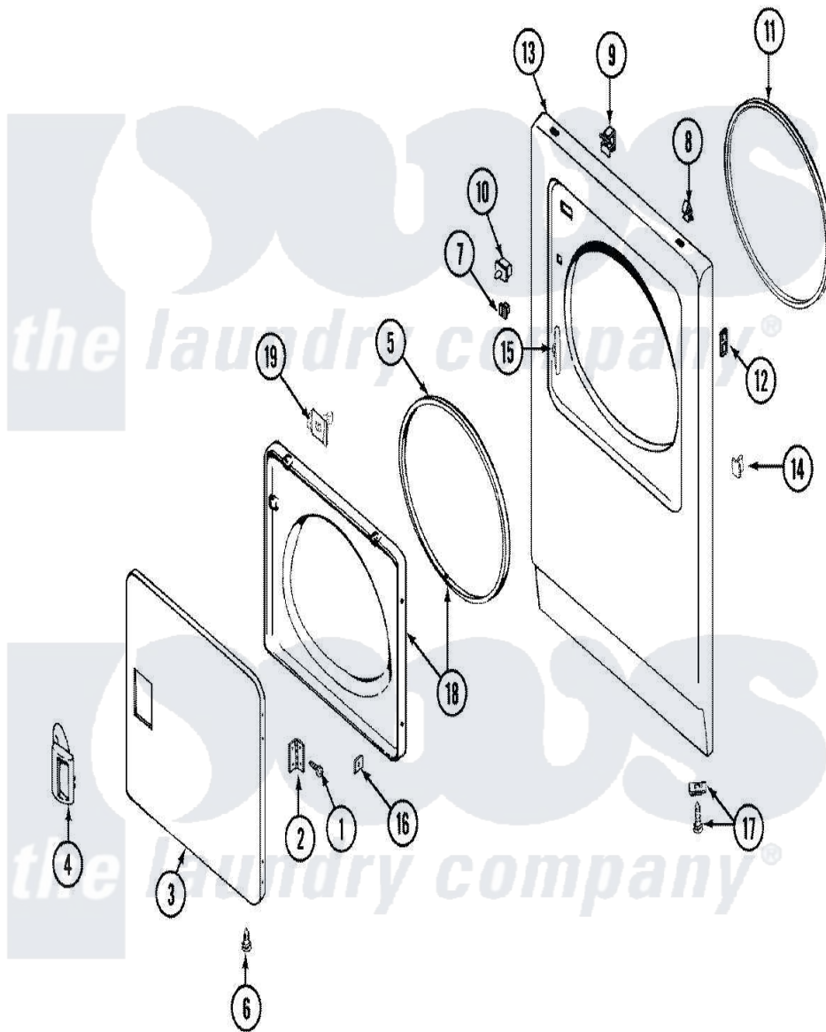
Maytag Residential Maytag LDE9804ACL Dryer Parts Parts Diagram 04 - DOOR Click on the part number to view part
