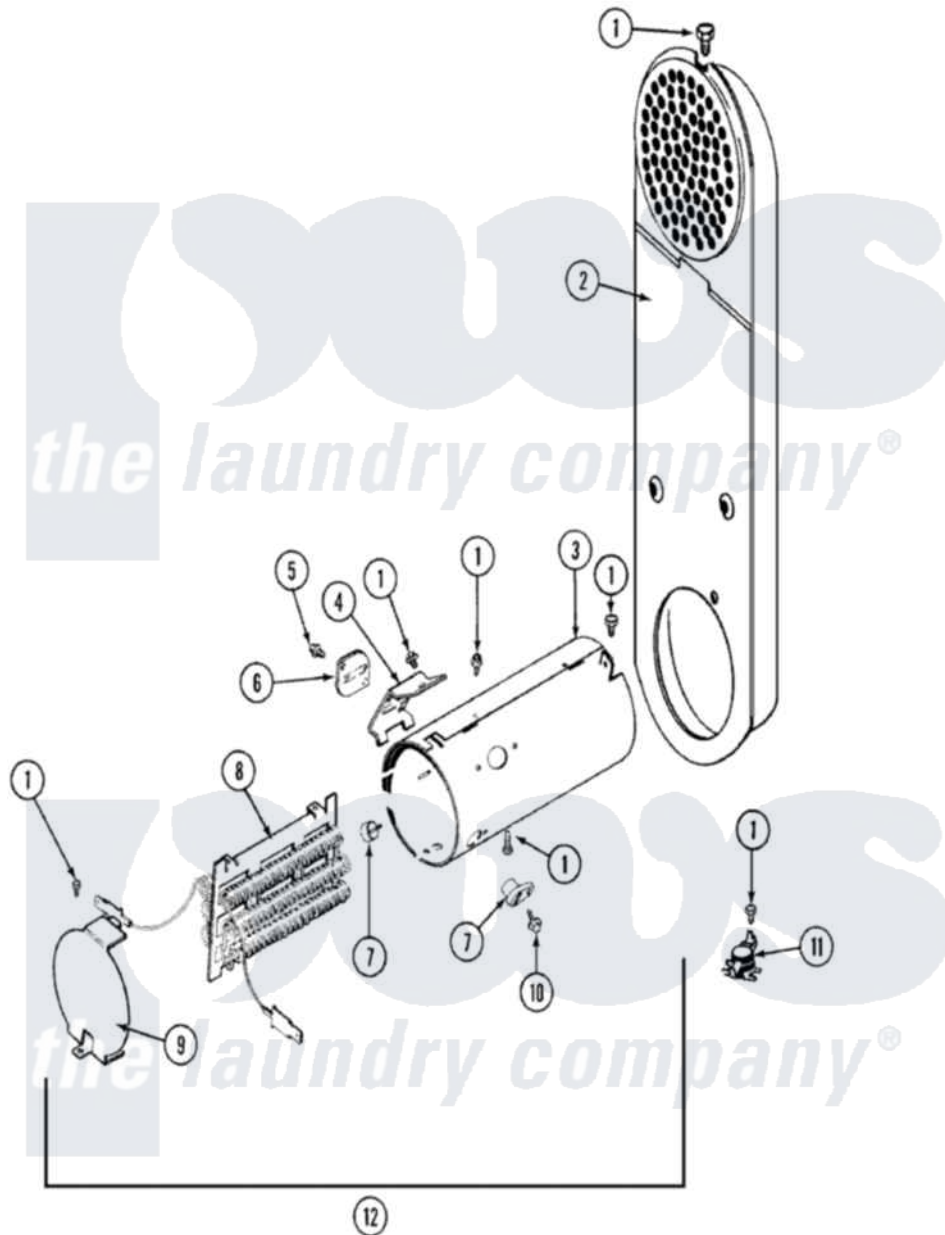
Maytag Residential Maytag LDE9804AEE Dryer Parts Parts Diagram 06 - HEATER Click on the part number to view part
