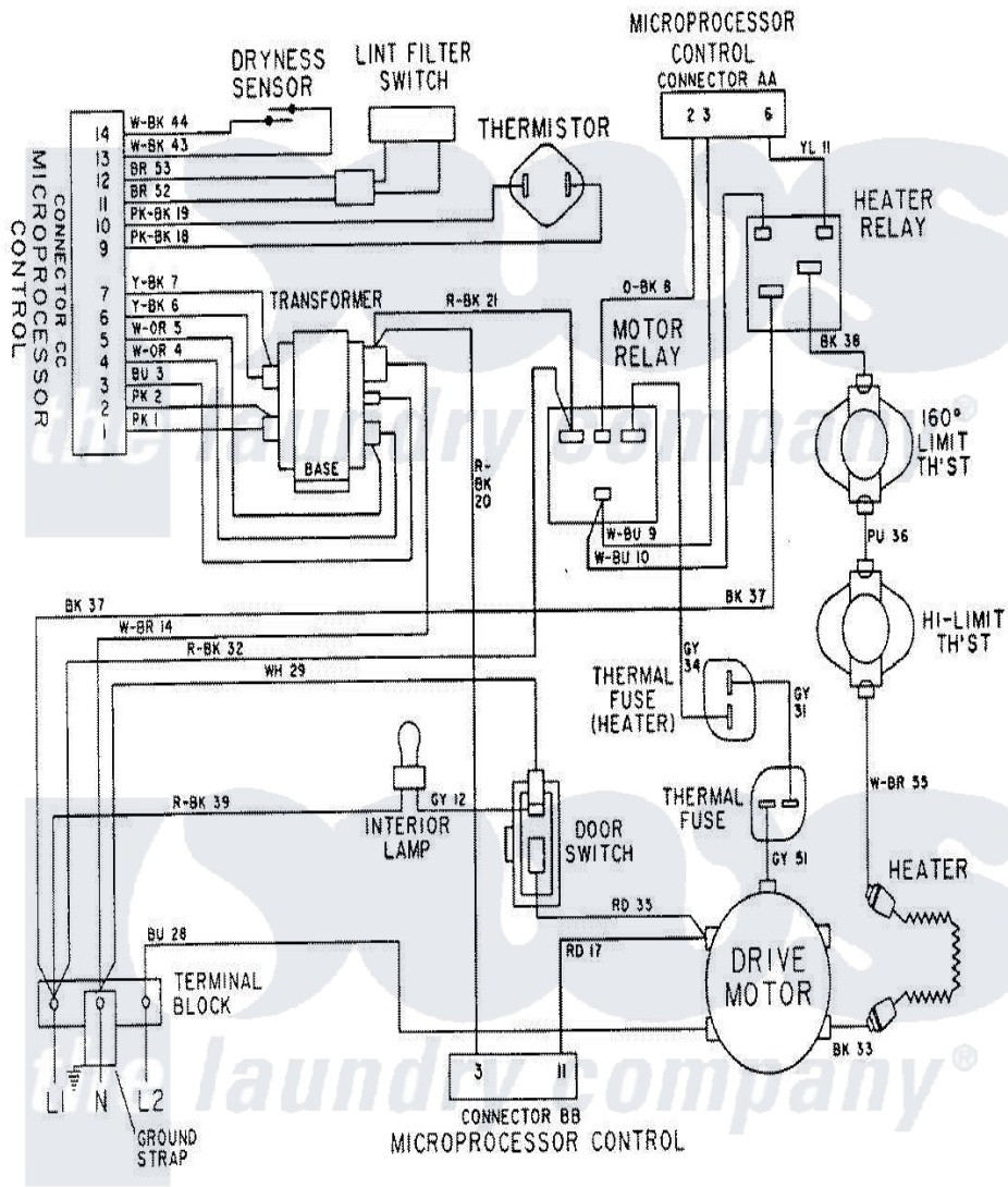
Maytag Residential Maytag LDE9904ACL Dryer Parts Parts Diagram 09 - WIRING INFORMATION-LDE9904ACx Click on the part number to view part
