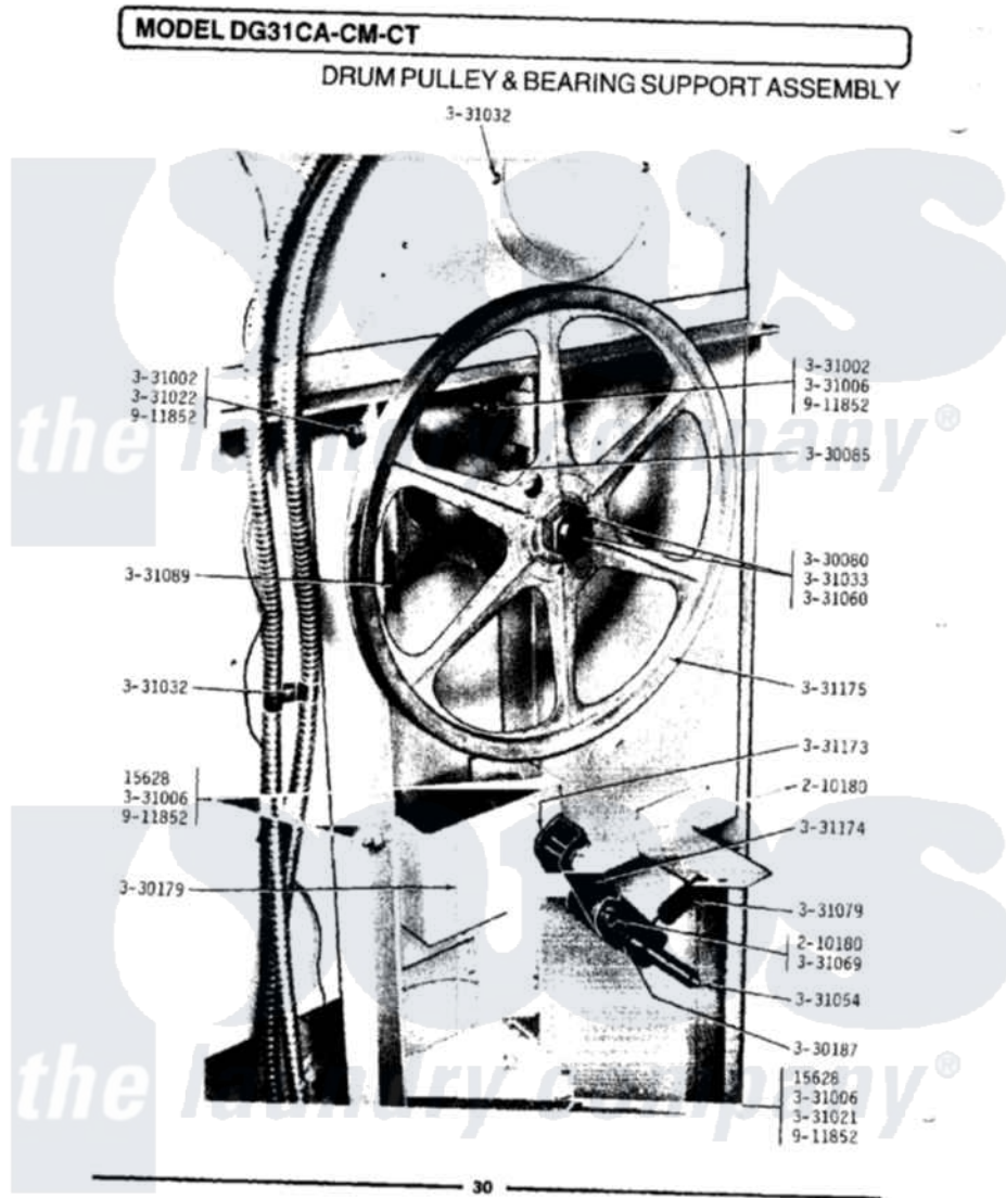
Maytag Residential Maytag LDG31CM Dryer Parts Parts Diagram 12 - DRUM PULLEY & BEARING SUPPORT ASSEMBLY
