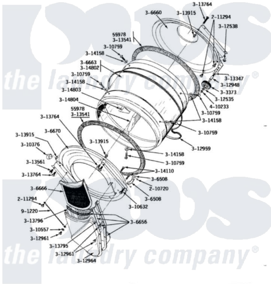
Maytag Residential Maytag LDG382 Dryer Parts Parts Diagram 06 - LINT SCREEN, TUMBLER (FRONT & BACK) Click on the part number to view part
